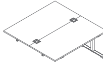
BRN16 1600 / 1600 / 740 87.2 kg
